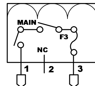
MAIN RELAY
