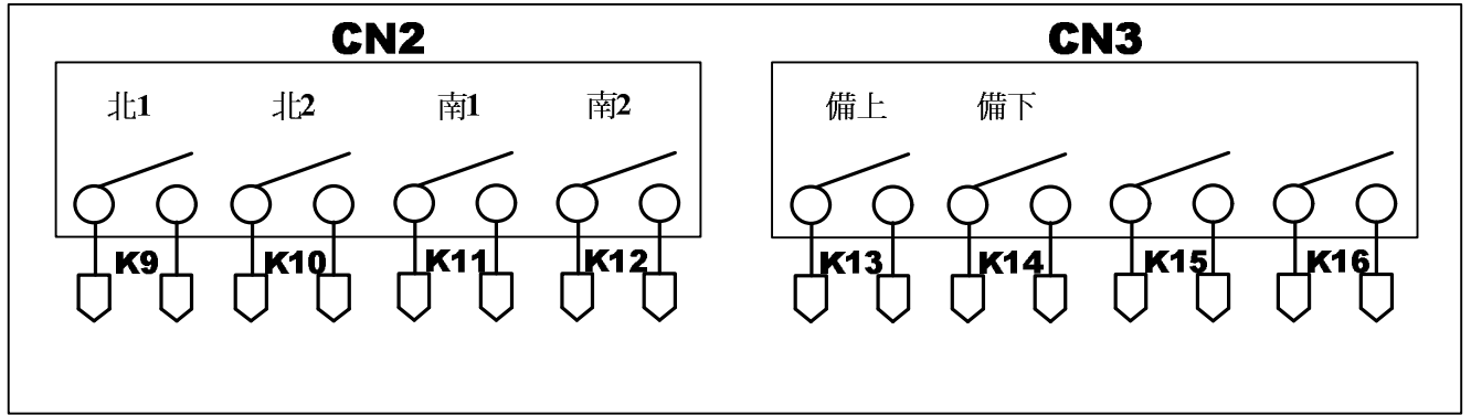
Relay Card 2
