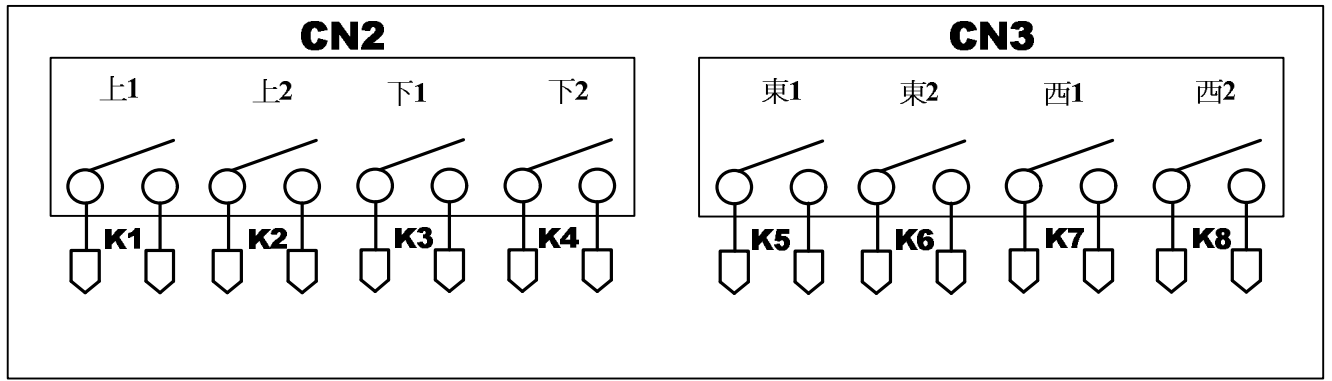
Relay Card 1
