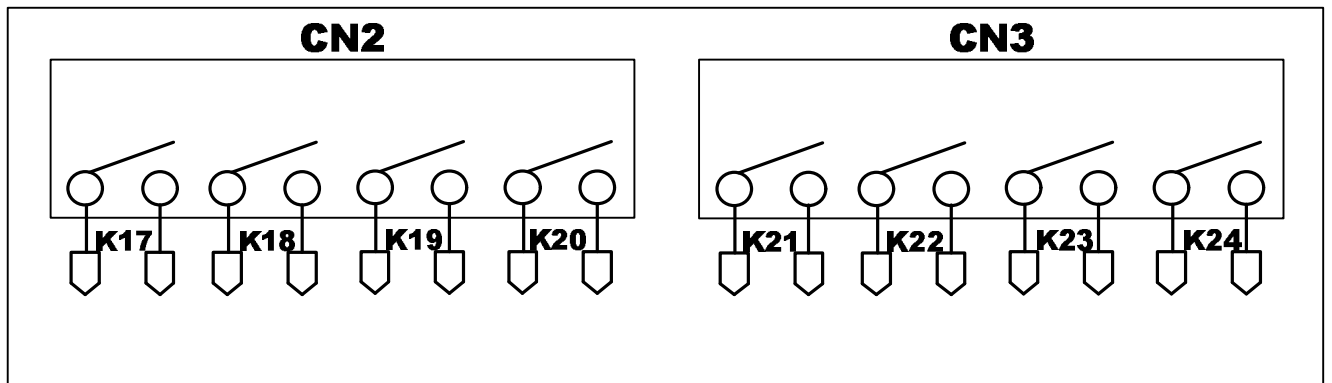
Relay Card 3
